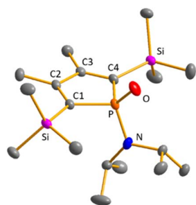
Fig. 12 Molecular structure of phosphole oxide 34a in the crystal. Thermal ellipsoids at 50% probability. Hydrogen atoms are omitted for clarity. Selected atomic distances [pm] and angles [°]: C 1 –C 2 135.42 (10), C 2 –C 3 151.31 (11), P–C 1 180.46 (8), P–O 148.78 (6).
