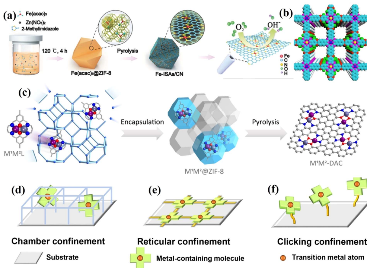
Fig. 4 (a) Schematic illustration of the formation of Fe-ISAs/CN. (b) Top views of a graphical representation of the eclipsed stacking of \text{CuPcF}_8\text{-CoNPC-COF} . (c) Schematic illustration of the synthesis of DACs via a macrocyclic precursor-mediated encapsulation-pyrolysis process. (d-f) Different confinement strategies for fabricating M-N-C SACs. (a) Reproduced with permission. 61 Copyright 2017, Wiley-VCH. (b) Reproduced with permission. 63 Copyright 2021, American Chemical Society. (c) Reproduced with permission. 37 Copyright 2023, American Chemical Society. (d-f) Reproduced with permission. 64 Copyright 2022, American Association for the Advancement of Science.
