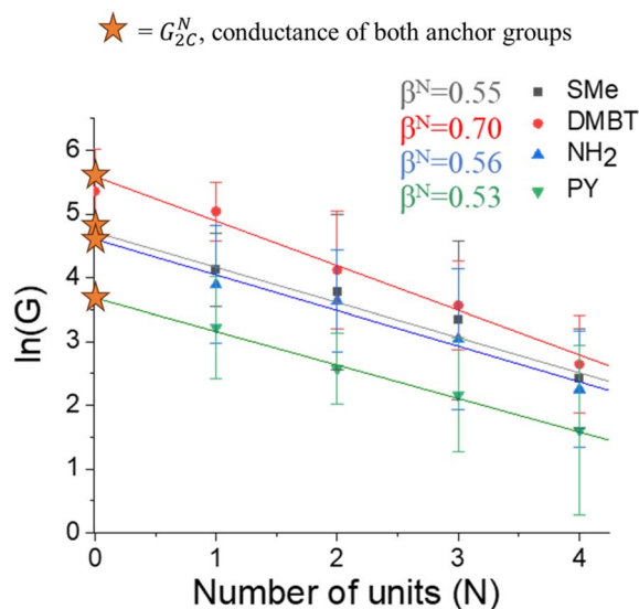
Fig. 54 Plot of the most probable experimental conductance values \ln(G) versus number of units -[\text{C}\equiv\text{C}-] , N , from STM-BJ measurements of the compounds shown in Fig. 53, conducted in mesitylene. 38
