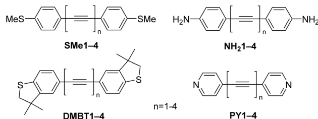
Fig. 53 The structures of the polyynes used to provide estimates of the polyindyl backbone parameters, b_B . 38
