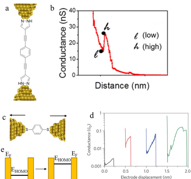
Fig. 37 (a) Schematic of 1,4-bis(1H-pyrazol-4-ylethynyl)benzene junction; (b) a representative G - s trace obtained for 1,4-bis(1H-pyrazol-4-ylethynyl)benzene with high and low conductance point; (c) schematic of a BDT molecular junction; (d) a representative G - \Delta z trace of BDT with spike in conductance; (e) schematic energy diagram demonstrating how the energy of the HOMO changes relative to E_F of the electrodes as electrode separation increases. Figures adapted with permission from ref. 117 and 118. Copyright 2018, American Chemical Society. Copyright 2011, Springer Nature Limited.
