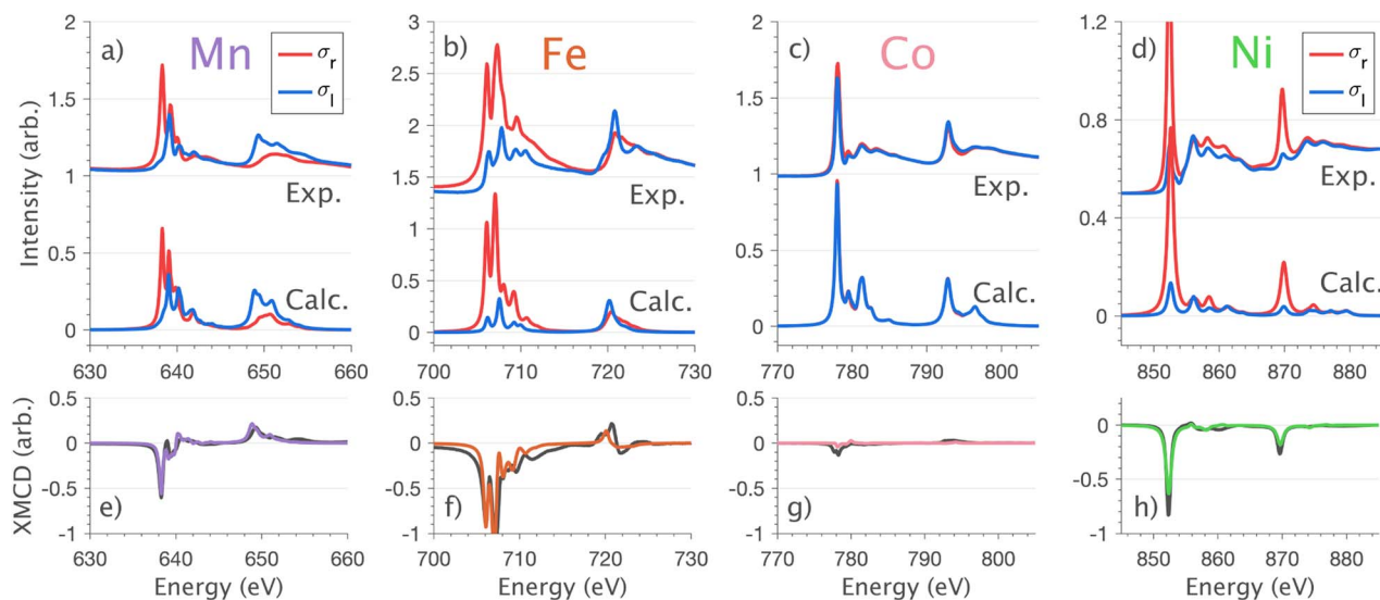
Fig. 8 Normal incidence ( \vec{E} \perp c ) single crystal L_{2,3} -edge XMCD measurements and calculations of \text{Li}_2(\text{Li}_{1-x}\text{TM}_x)\text{N} (where \text{TM} = \text{Mn, Fe, Co and Ni} ). (a–d) Circular polarisation absorption spectra \sigma_r (red) and \sigma_l (blue) with resultant (e–h) XMCD ( \sigma_r - \sigma_l ) spectra; experimental (black) and charge-transfer multiplet calculations (colour) measured at 21 K and 14 T.
