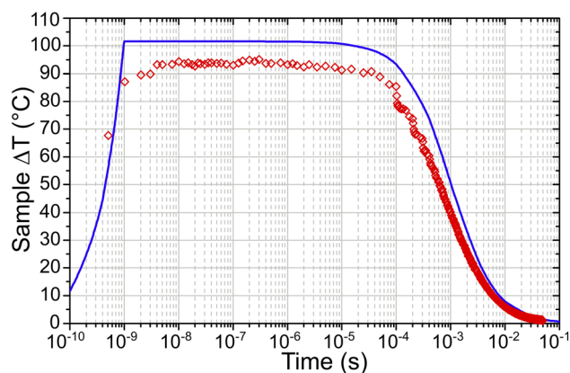
Fig. 8 Average sample temperature across the probed region vs. time for a temperature jump from 175 °C T_{Act} as determined experimentally (red) and from simulations (blue). The simulation uses the best estimates for input parameters.
