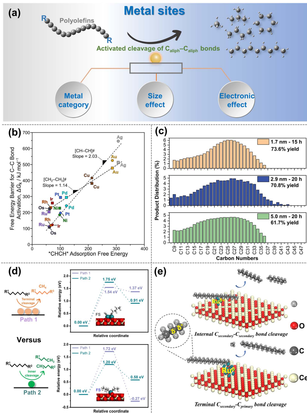
Fig. 4 (a) Schematic diagrams of the upgrading of polyolefins when C_{aliph}-C_{aliph} bonds are activated over the metal sites. (b) Free-energy barriers \Delta G_k for C_{aliph}-C_{aliph} bond activation in ^*CHCH^* (circles) and ^*CH_2CH_2^* (squares) as a function of ^*CHCH^* adsorption free energies over various metal sites (593 K, 1 bar H_2 ). Data collected from ref. 97. Copyright 2019 American Chemical Society. (c) Carbon number distributions of hydrogenolysis of polyolefins over size-controlled Pt nanoparticles, data collected from ref. 76 and copyright 2022 American Chemical Society. (d) Summarized cleavage modes of polyolefin on conventional SAC and nanocluster catalyst, reproduced with permission from ref. 100 and copyright 2023 Science Partner Journals. (e) Proposed reaction mechanism of polyethylene hydrogenolysis over different Ru chemical states of Ru/CeO 2 catalysts. Data collected with permission from ref. 22. Copyright 2023 Wiley.
