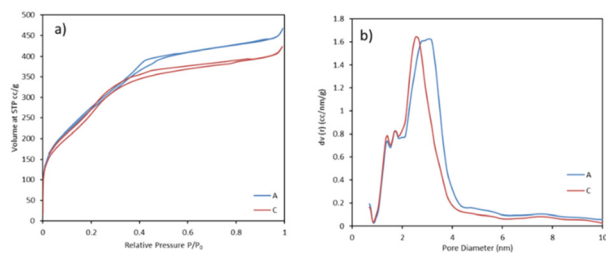
Fig. 4 a) BET adsorption and desorption isotherms and b) pore size distribution calculated by the DFT method (A = reaction performed without pulse, T_G = 55\text{ }^\circ\text{C} , C = pulse of methanol given for 5 s@88 ml \text{min}^{-1} , T_G = 45\text{ }^\circ\text{C} ).
