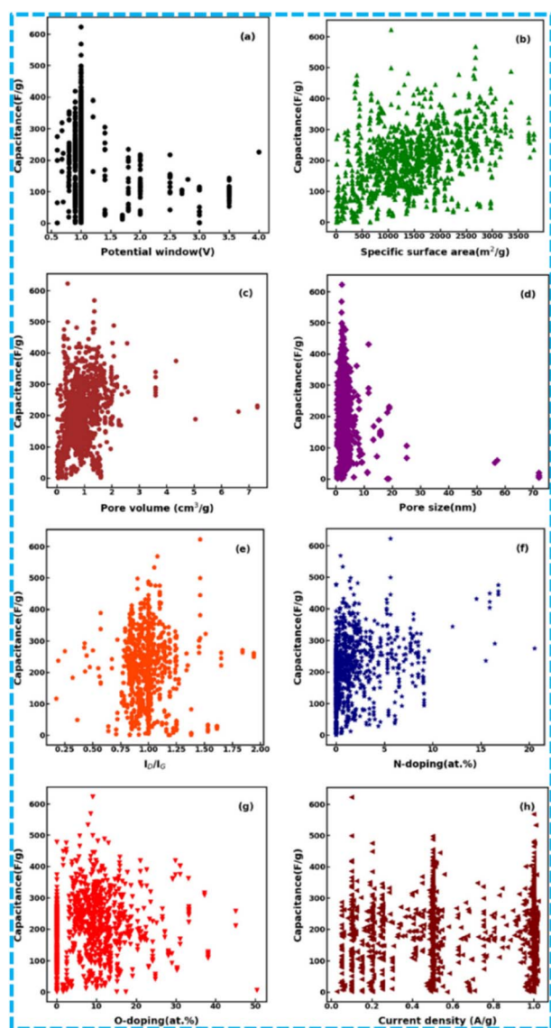
Fig. 22 (a–h) Illustration of the relationship between various input features and specific capacitance. This figure has been reproduced from ref. 155 with permission from Nature, copyright 2023.
