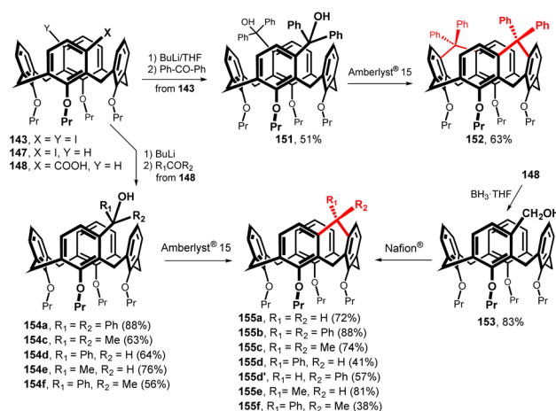
Fig. 39 Upper rim-bridged calix[4]arenes by intramolecular Friedel–Crafts alkylation.
