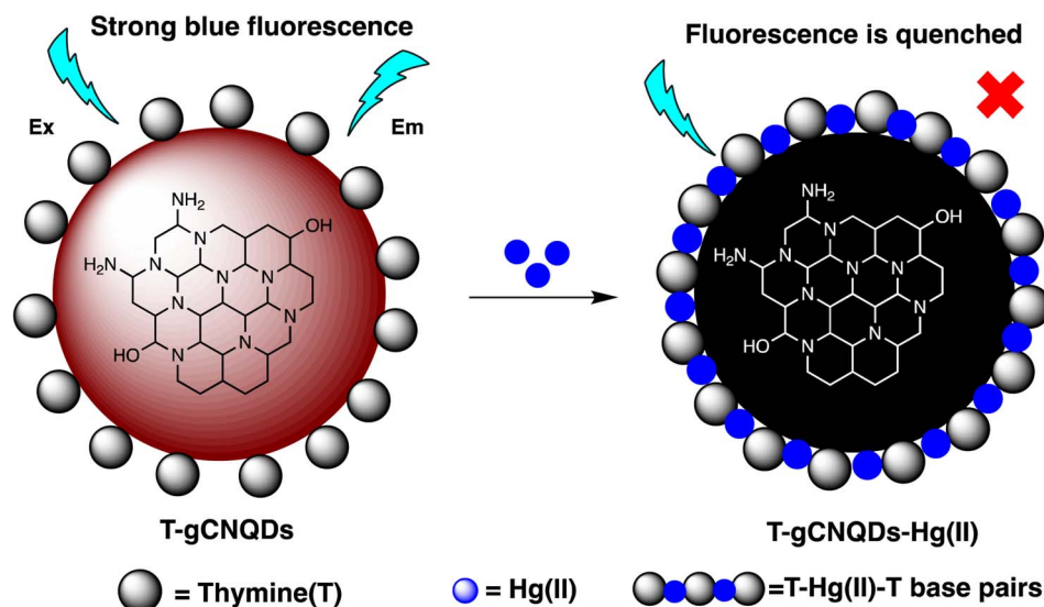
Scheme 10 Schematic representation of \text{Hg}(\text{II}) binding on T-gCNQDs surface.
