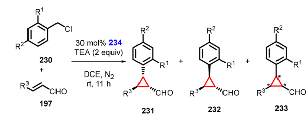
Scheme 51 MIRC cyclopropanation of benzyl chlorides and \alpha,\beta -unsaturated aldehydes.
