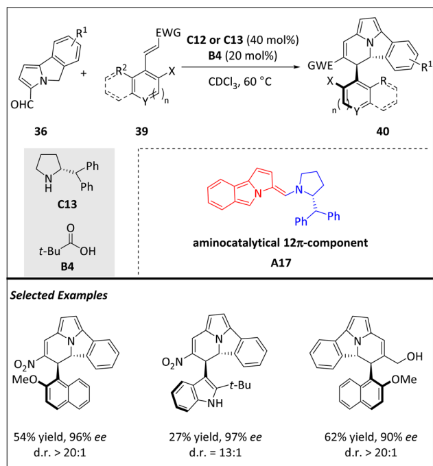
Scheme 13 Enantioselective intermolecular [12 + 2] cycloadditions for the construction of C(sp 2 )–C(sp 3 ) atropisomers.
