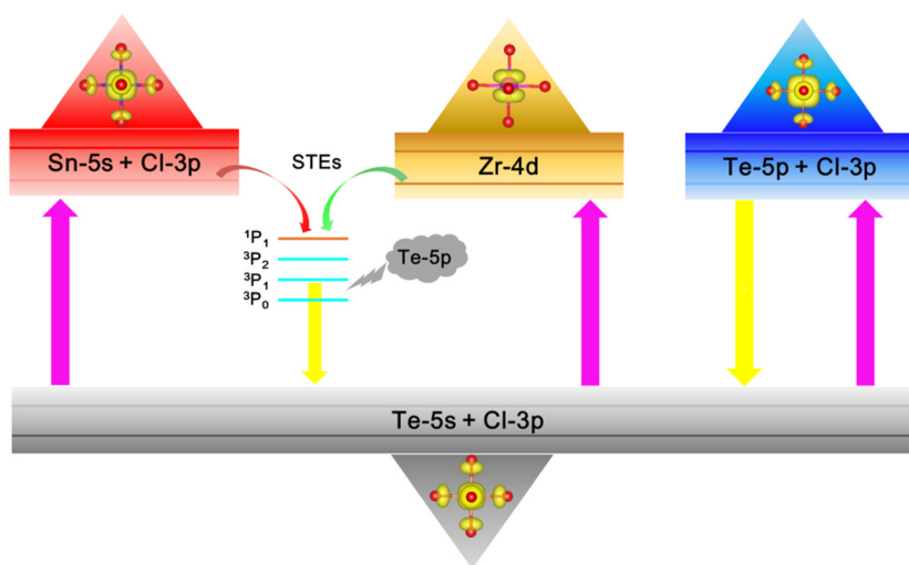
Fig. 8 Schematic diagram of the luminescence mechanism of \text{Te}^{4+} -doped metal VODPs with different M-sites.
