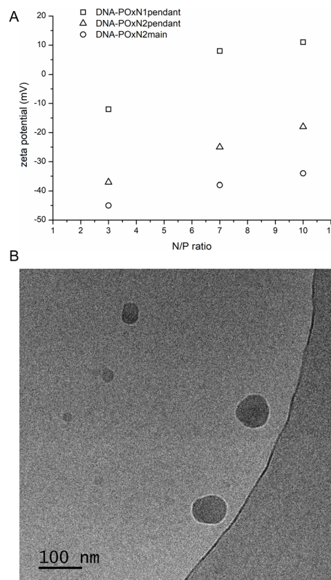
Fig. 6 \zeta of DNA-POxN1pendant, DNA-POxN2pendant and DNA-POxN2main as a function of N/P ( 7.5 \text{ mg mL}^{-1} , 25^\circ\text{C} ) (A); cryo-TEM images of DNA-POxN2pendant at N/P = 7 (B).
