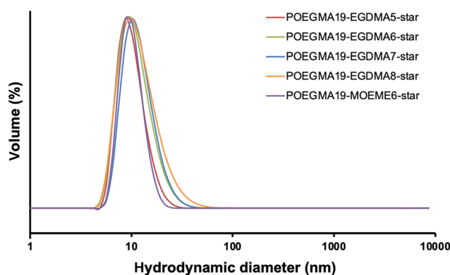
Fig. 2 DLS volume weighted diameter distribution for all “arm-first” PEOGMA 19 -EGDMA x -star and PEOGMA 19 -MOEME y -star star polymers (1 mg mL -1 in deionized water).
