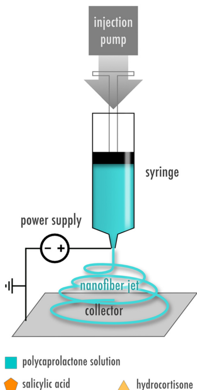
Fig. 1 A schematic illustration demonstrating the electrospinning process for single-layer and layer-by-layer fiber mats, with and without active ingredients. The part on the left illustrates the electrospinning process, where a polymer solution is injected into an electric field through a syringe using a pump, leading to the deposition of polymer fibers on the collector. The center of the figure depicts the layered structure of electrospun materials, which can combine drug-free and drug-loaded layers. An electrospun dressing is produced, shown on the right, that can consist of either a single layer (blue) or multiple layers (orange, yellow, blue).
