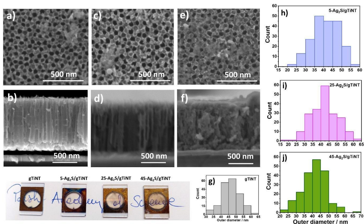
Fig. 3 SEM images of (a and b) 5- \text{Ag}_2\text{S}/\text{gTiNT} , (c and d) 25- \text{Ag}_2\text{S}/\text{gTiNT} , (e and f) 45- \text{Ag}_2\text{S}/\text{gTiNT} , and size distribution of \text{TiO}_2 nanotubes outer diameter (g) gTiNT, (h) 5- \text{Ag}_2\text{S}/\text{gTiNT} , (i) 25- \text{Ag}_2\text{S}/\text{gTiNT} , (j) 45- \text{Ag}_2\text{S}/\text{gTiNT} .
