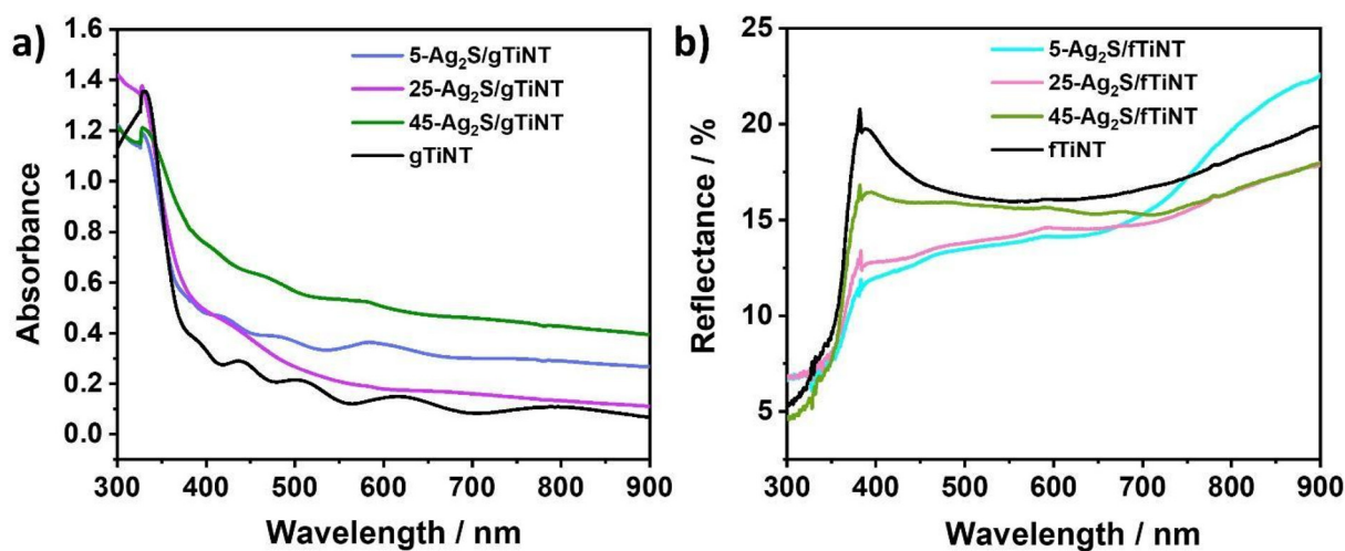
Fig. 4 UV-vis (a) absorbance spectra for \text{Ag}_2\text{S} -coated and non-coated gTiNT and (b) reflectance spectra for \text{Ag}_2\text{S} -coated and non-coated fTiNT.
