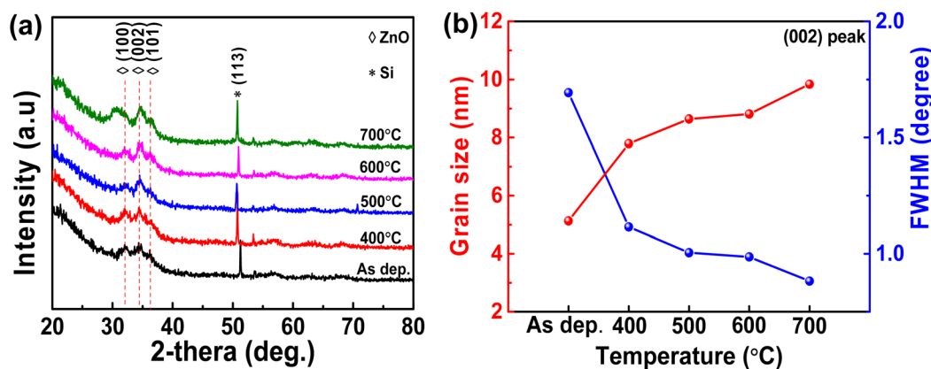
Fig. 3 (a) X-Ray diffraction spectra of \text{HfO}_2/\text{ZnO} films without and with thermal annealing from 400 °C to 700 °C. (b) Dependence of the full width at half maximum (FWHM) and average grain size of \text{HfO}_2/\text{ZnO} films on annealing temperature.
