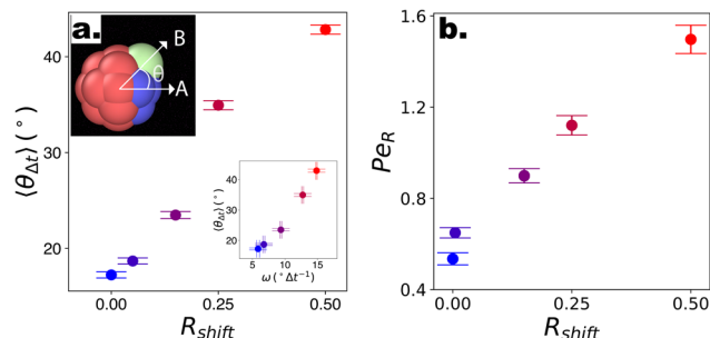
Fig. 4 Swimming dynamics of CF microswimmers with respect to their cap orientation, in the absence of gravity and bounding substrates, as a function of introduced shape asymmetry R_{\text{shift}} (colour coded from blue to red with increasing R_{\text{shift}} ). (a) Increasing divergence \langle\theta\rangle in the internal body axis and the observed swimming direction is measured with increasing R_{\text{shift}} . We note that the values of \langle\theta\rangle are a function of the time-step evaluated (here, \sqrt{D_T\Delta t}/R \sim 0.13 , where D_T is the constant obtained for a passive sphere with R_{\text{shift}} = 0 ). Inset: linear growth in \langle\theta\rangle with \omega values fitted from the microswimmers’ MSAD (see ESI, Fig. S6†). Graphical inset: angle \theta between the swimming direction and internal body axis, as defined in the text. The particle depicted has R_{\text{shift}} = 0.5 . (b) Rotational Péclet number as a function of R_{\text{shift}} for \Delta t = 1 . Error bars either indicate the standard error of the mean, or for the fits of \omega and D_R are obtained from the co-variance matrix, accounting for error propagation where relevant, from 1001 frames (sub-sampled from 50 000 simulation steps).
