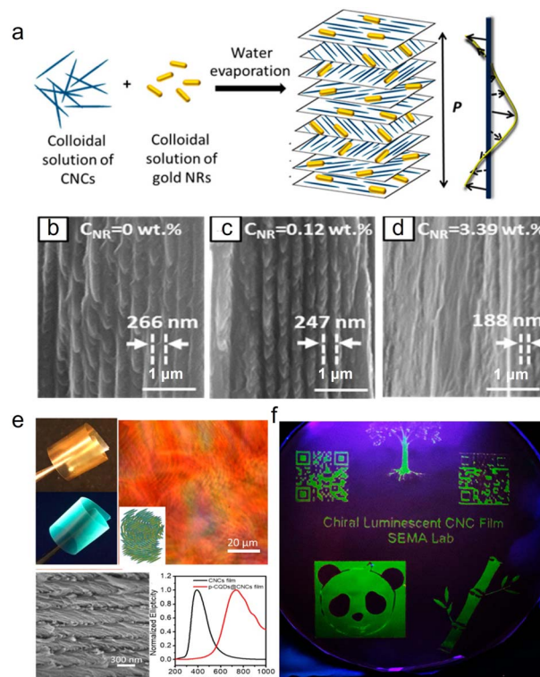
Fig. 7 (a) Schematic of the preparation of the composite chiroptical plasmonic film by mixing aqueous suspensions of CNCs and GNRs. Representative SEM images of the cross-section of the CNC/GNR films at NR concentrations of (b) 0, (c) 0.12 wt%, and (d) 3.39 wt%. 114 Copyright 2014, American Chemical Society, (e) Characterization of the chiral luminescent CQDs/CNCs film: POM image, SEM image, and CD spectra. (f) Patterned chiral luminescent CQDs/CNCs films with 10 cm diameter at 365 nm UV light. 119 Copyright 2019, American Chemical Society.
