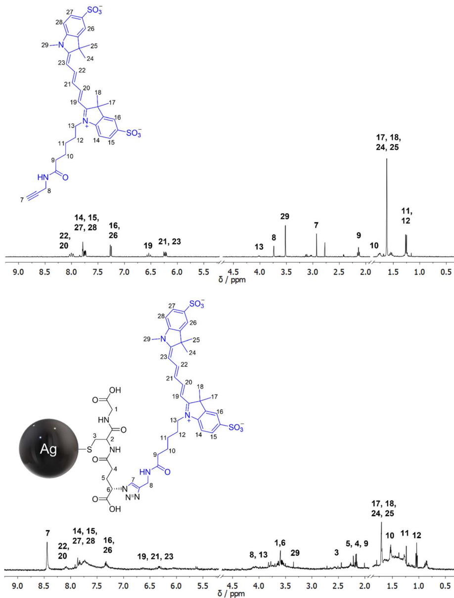
Fig. 6 1 H NMR spectra of the dissolved (free) alkyne-terminated dye sulfo-Cy5 (top) and the dye clicked to glutathione-azide-terminated silver nanoparticles (bottom). The spectrum of sulfo-Cy5 (blue) on the nanoparticles is rather crowded due to inherent peak broadening and the presence of the primary ligand glutathione (black). Thus, the peak assignments are uncertain in most cases. However, the alkyne proton of the dissolved dye (H7 at 2.93 ppm) and the triazole proton of the clicked dye (H7 at 8.44 ppm) are clearly visible, confirming the successful click reaction. The spectra were recorded at 600 MHz in 90% H 2 O/10% D 2 O at pH 8.0. The water suppression signal was cut out (4.79 ppm). In the bottom spectrum, a large solvent peak at 1.90 ppm was cut out.
