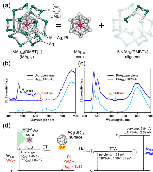
Fig. 14 (a) Schematic illustration of MAg 24 (M = Ag, Pt). (b) and (c) Photoluminescence spectra for deaerated solution of Ag 25 /emitter and PtAg 24 /emitter (emitter = perylene or TIPS-Ac), respectively, excited by 640 nm. (d) Relaxation process of excited MAg 24 and energy diagram of TTA-UC in the MAg 24 /emitter system. Reproduced from ref. 74 with permission from Wiley-VCH GmbH, Copyright 2020.
