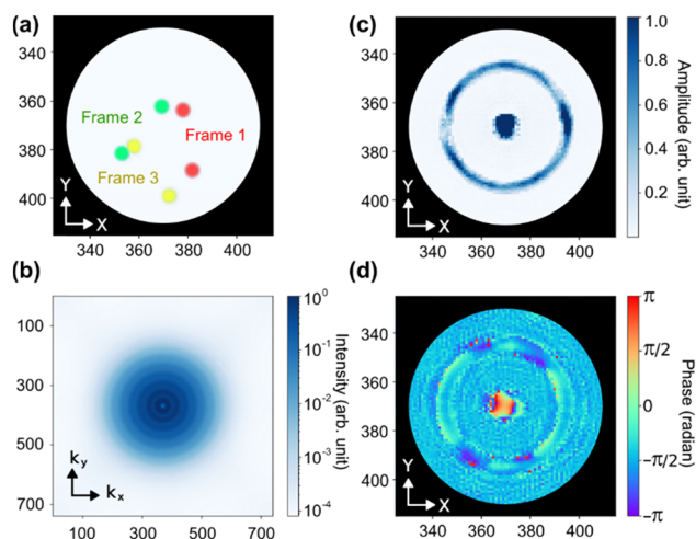
Fig. 4 CIDI of randomly oriented polaron pairs. (a) Image of a pair of polarons with fluctuating mean position and arbitrary orientation in two dimensions is shown for three frames. The three different locations are represented by three different colours. (b) Fluctuation spectrum of the pair of polarons with arbitrary orientation retrieved using CIDI. (c) Amplitude and (d) phase image recovered using CDI from the pattern in panel b. A central peak and outer ring are recovered; the width of the central peak and radial width of the outer ring match the size of the polarons, while the relative phase of \pi corresponds to the relative phase of the two polarons. The separation of the polarons matches the radius of the ring.
