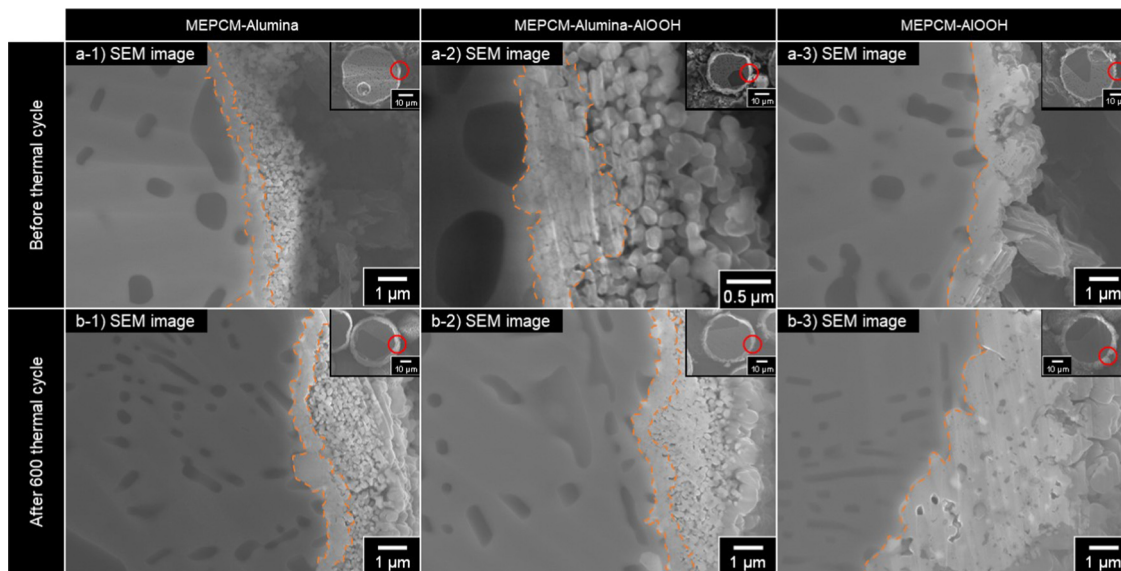
Fig. 9 Cross-sectional SEM images of the MEPCMs before and after 600 cyclic tests. Samples include MEPCM-alumina, MEPCM-alumina-AIOOH, and MEPCM-AIOOH. Orange lines indicate the interface between the PCM core and its shell.
