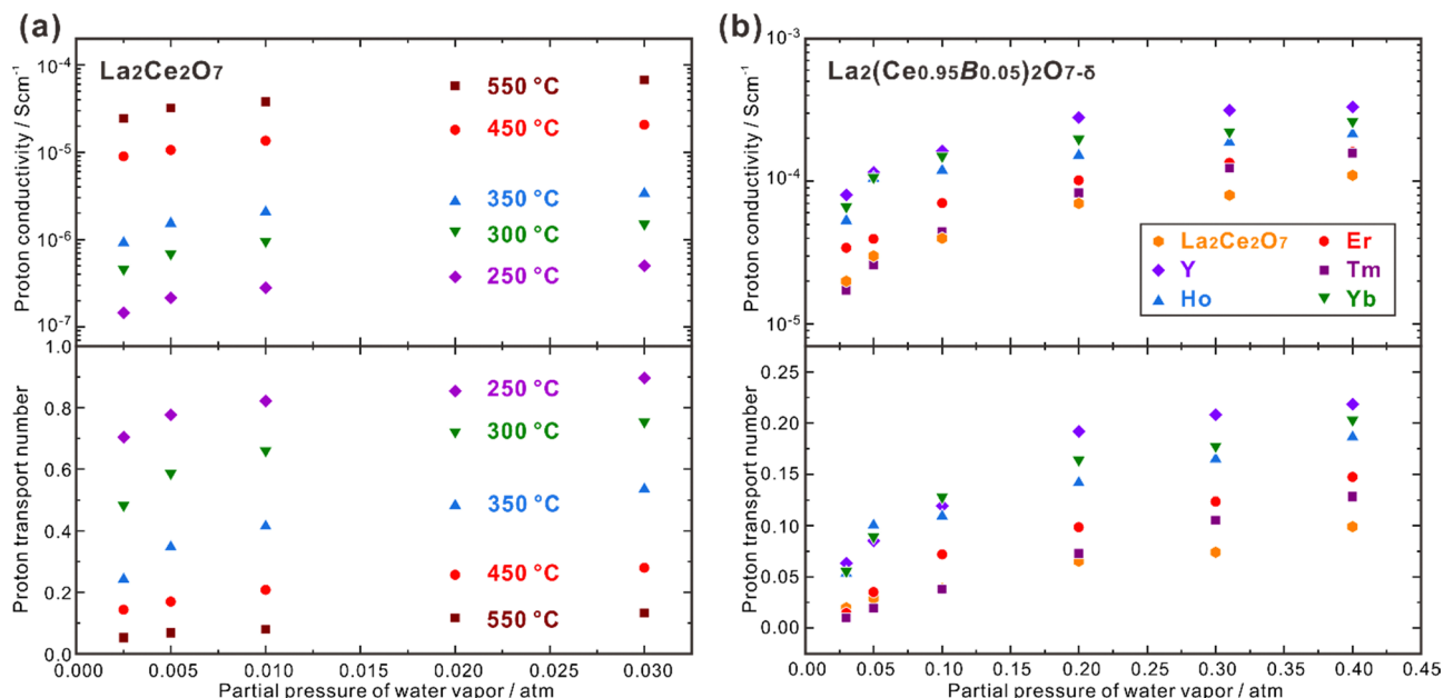
Fig. 4 Proton conductivity and proton transport number of (a) \text{La}_2\text{Ce}_2\text{O}_7 in wet air, 76 and (b) \text{La}_2(\text{Ce}_{0.95}\text{B}_{0.05})_2\text{O}_{7-\delta} ( \text{B} = \text{Y}, \text{Ho}, \text{Er}, \text{Tm} and \text{Yb} ) at 600 °C in wet oxygen plotted against p_{\text{H}_2\text{O}} . 75
