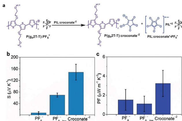
Fig. 54 (a) Structure of the P(g_42T-T) with \text{croconate}^{2-} . Thermoelectric parameters of chemically doped and ion exchange P(g_42T-T) films. (b) Seebeck coefficients ( S ) and (c) power factors ( PF ) of P(g_42T-T):PF_6^- , P(g_42T-T):PF_6^- , low, and P(g_42T-T):croconate^{2-} thin films. Reproduced from ref. 234 with permission from Wiley-VCH, Copyright [2023].
