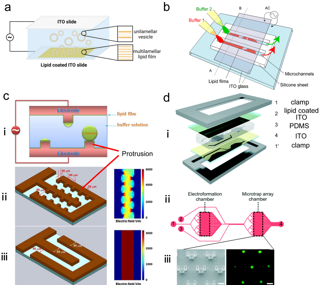
Fig. 14 On-chip electroformation. a ) Mechanism of conventional electroformation. Lipid film is coated on the surface of the electrode, usually indium tin oxide (ITO) slides. An electric field is applied across the lipid film and surrounding buffer. The lipids interact with the aqueous solution and electric field by “peeling off” the electrode surface in layers and self-assembling into vesicles. b ) Schematic of electroformation in a microfluidic device developed by Kuribayashi et al. The glass slides were coated with ITO electrodes and clamped a silicone sheet containing microfluidic channels where the electroformation occurred. Reproduced from ref. 201 with permission from IOP Publishing, copyright [2006]. c ) (i) Schematic diagram of on-chip giant vesicles electroformation process developed by Wang et al. (ii) Protruding microelectrode array with spatially non-uniform electric field. And (iii) planar electrode array with uniform electric field. Reproduced from ref. 202 with permission from Elsevier, copyright [2013]. d ) (i) Exploded 3D diagram of microfluidic electroformation device developed by Paterson et al. , showing 1,1' clamps; 2 lipid-coated ITO-coated slide; 3 PDMS sheet and 4 ITO-coated slide, arranged into a glass-PDMS-glass sandwich. (ii) Plan view of chip design (top), showing the electroformation and microtrap analysis chambers, connected by microfluidic channels (1), also depicted are the (2) wash and (3) peptide channels, as well as a collective outlet for waste (4). (iii) The microtrap array region was fabricated to capture GUVs for imaging analysis, of which the SEM image (bottom left, scale bar represents 50 \mu\text{m} ) and fluorescent image of GUVs within it (bottom right, scale bar represents 50 \mu\text{m} ) are presented. Reproduced from ref. 203 with permission from the Royal Society of Chemistry, copyright [2014].
