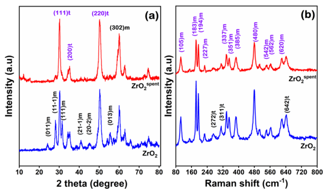
Fig. 2 (a) X-ray diffraction patterns of ZrO_2 and (b) Raman spectra of ZrO_2 .
