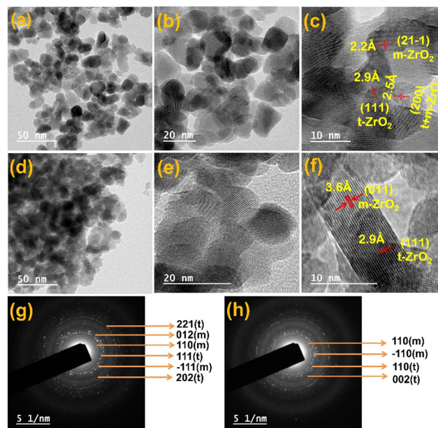
Fig. 3 HR-TEM images (a) fresh and (d–f) spent pure zirconium oxide ( ZrO_2 ); catalysts. The SAED images of (g–h) of fresh and spent ZrO_2 .
