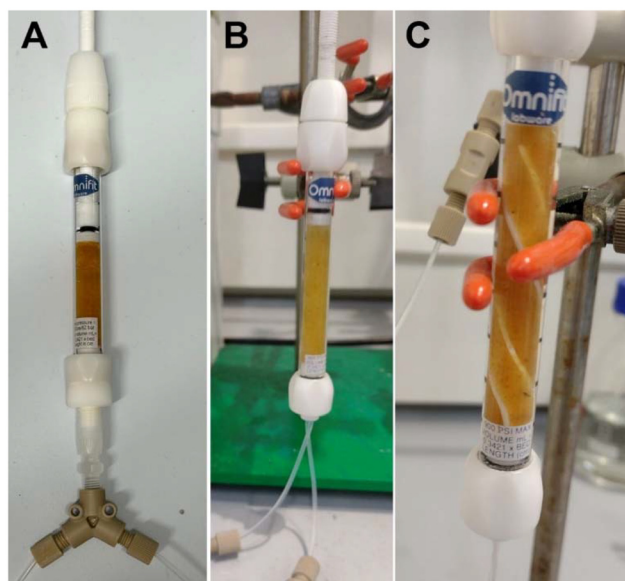
Fig. 1 Catalyst bed design. (A) Initial set up. Imine and thiol are premixed before entering the catalyst bed. (B) Second design, no premixing before the packed bed reactor. (C) Final setup with spiral mixing element installed inside the packed-bed reactor.
