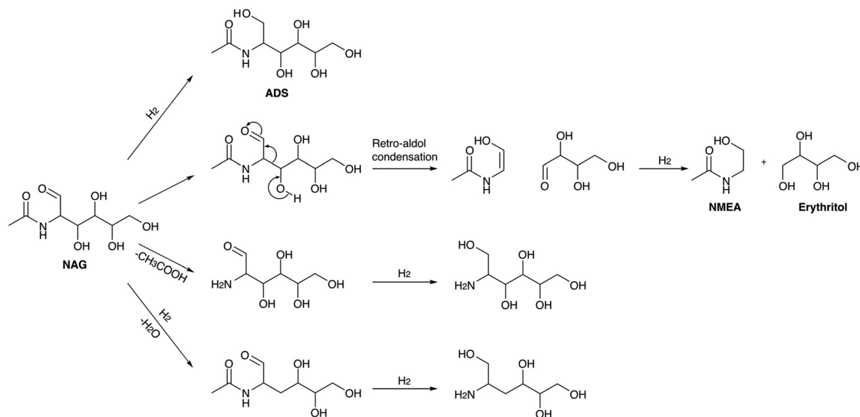
Scheme 6 Reaction pathways for the formation of C4, C6 polyols and NMEA from NAG.
