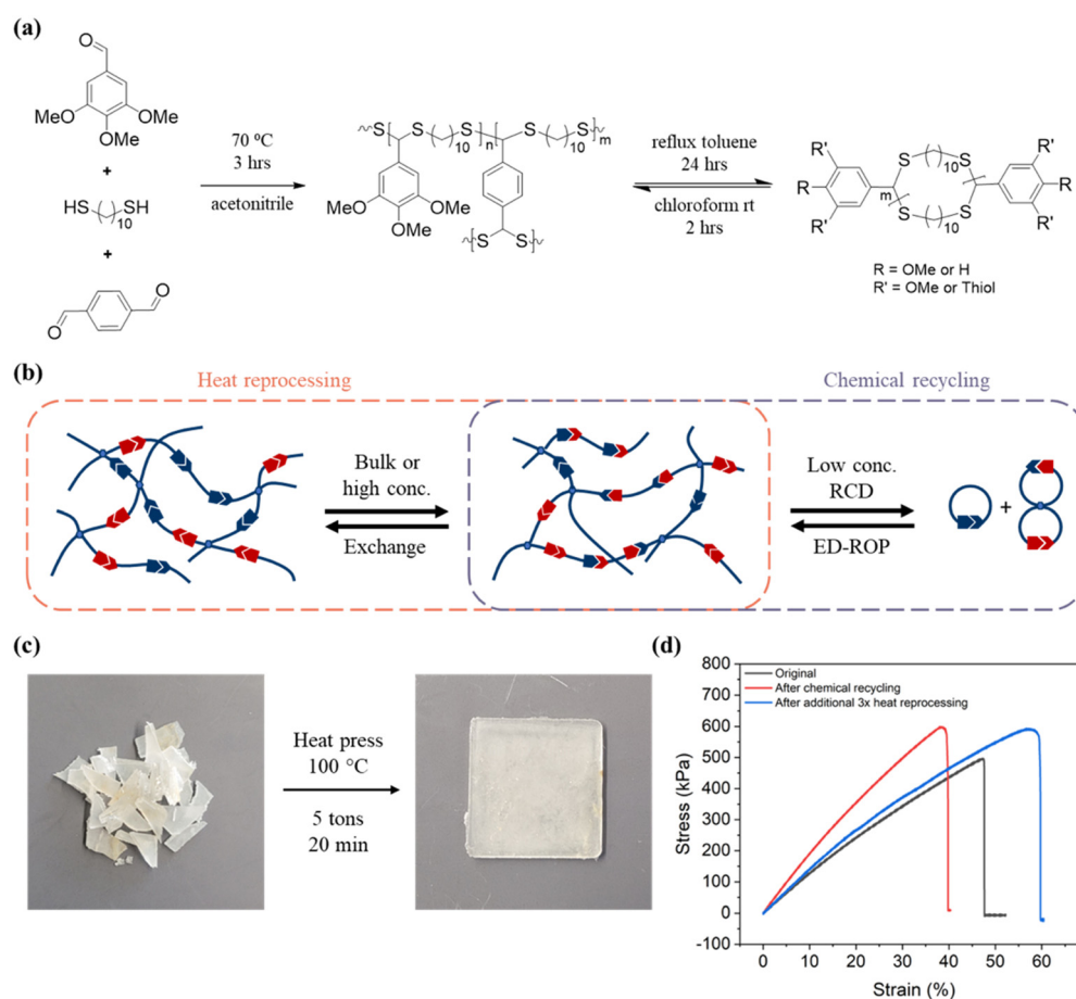
Fig. 17 Reprocessability and mechanical properties of the crosslinked PDTA network. (a) Synthesis of cPDTA and recycling process. (b) Schematic illustration of the reprocessing and recycling mechanisms. (c) Pictures of heat pressing processing. (d) Stress-strain curves of the original network (black), immediately post-chemical reprocessing (red), and 3x mechanical recycling post-chemical reprocessing (blue). Reproduced from ref. 143 with permission from Wiley, copyright 2023.
