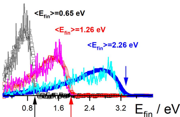
Fig. 8 H scattering from Au(111) at three incidence energies E_{in} . Experimental results (open squares) are compared to theory (solid lines): E_{in} = 3.33 \text{ eV} (blue), 1.92 \text{ eV} (red), and 0.99 \text{ eV} (black). Colored arrows mark the three incidence energies. Also shown are the average final translational energies, \langle E_{fin} \rangle . The scattering angles are \vartheta_i = 45^\circ , \vartheta_s = 45^\circ and \varphi_i = 0^\circ with respect to the [101] direction. Adapted from ref. 353 and used with permission under lic. no. 574300005425.
