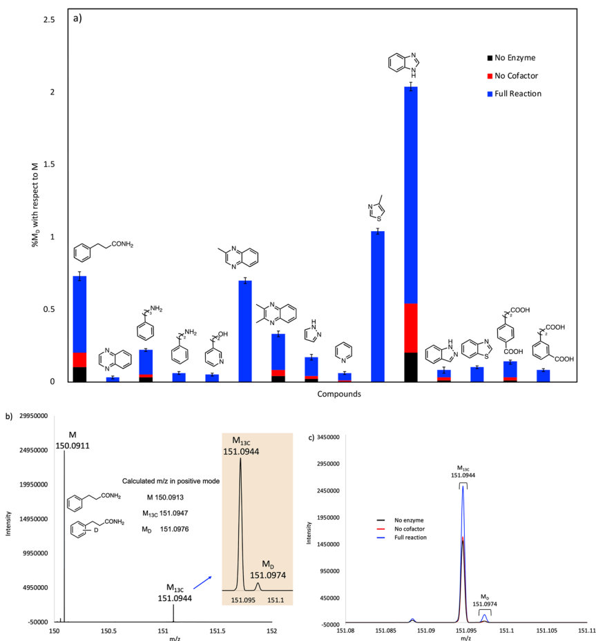
Fig. 3 (a) Plot showing solvent deuterium incorporation in various substrates catalyzed by purified, holo-FDC. Mol% deuterium incorporations ( M_D ) are shown relative to molecular ion (M) peak for each compound. (b) Mass spectrum showing the calculated and experimental M, M_{13C} and M_D peaks for 3-phenylpropanamide substrate. (c) Mass spectra for 3-phenylpropanamide of the experimental reaction, no enzyme, and no cofactor controls overlaid for comparison.
