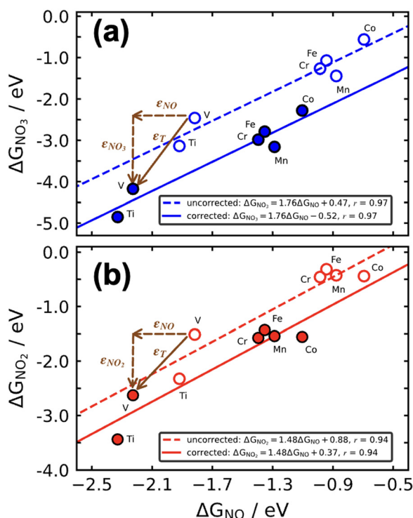
Fig. 15 Free energies of adsorption of ^*\text{NO}_3 (a) and ^*\text{NO}_2 (b) versus that of ^*\text{NO} on metallocporphyrins. Dashed lines and open circles correspond to uncorrected energies, solid lines and solid circles correspond to energies upon gas-phase corrections. Brown vectors on the V-containing porphyrin show the displacements introduced by the respective gas-phase errors. Reproduced from ref. 29, licensed under CC BY 4.0 ( https://creativecommons.org/licenses/by/4.0/ ).
