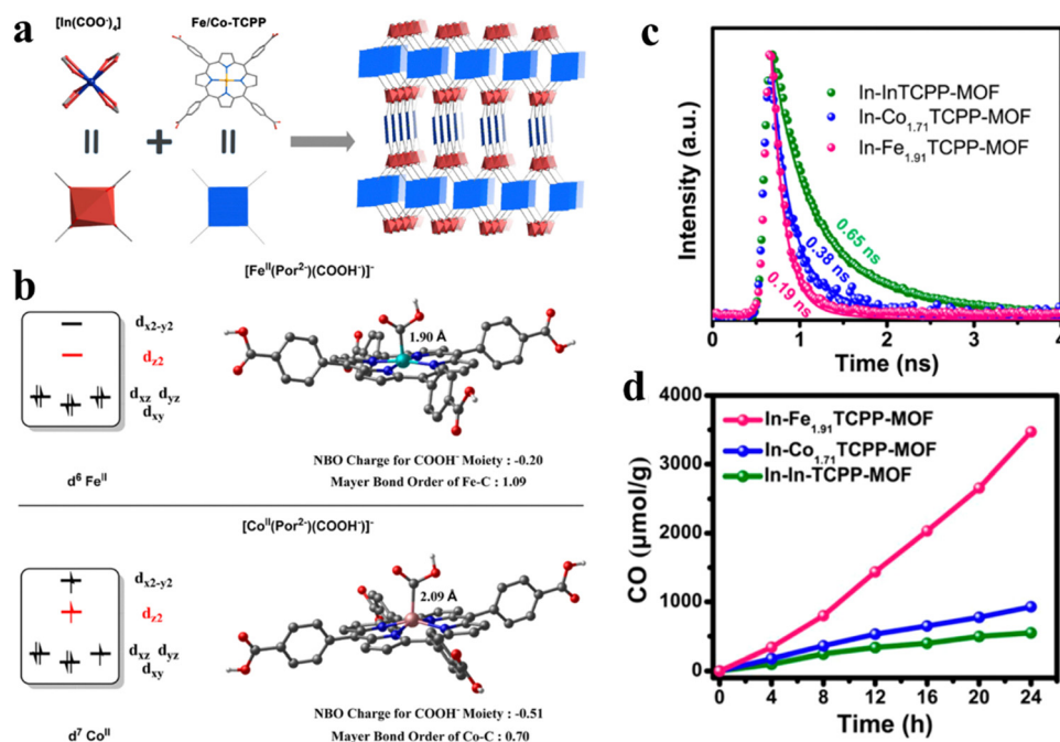
Fig. 11 (a) Synthesis and structure of In-Fe/CoTCPP-MOFs. (b) Influence of the electron configurations of the metal centers on metal-carbon interactions in [Fe II (Por 2- )(COOH - ) 2 ] - and [Co II (Por 2- )(COOH - ) 2 ] - . (c) Time-resolved PL decays of In-Fe 1.91 TCPP-MOF, In-Co 1.71 TCPP-MOF, and In-InTCPP-MOF under excitation at 440 nm. (d) Time profiles for the CO evolution catalyzed by In-Fe 1.91 TCPP-MOF, In-Co 1.71 TCPP-MOF, and In-InTCPP-MOF under irradiation with a 300 W xenon light source (>400 nm) in the presence of 0.1 M L-ascorbyl palmitate (L-AP) in ethyl acetate under 1 atm CO 2 . Reproduced from ref. 129. Copyright 2022 ACS.
