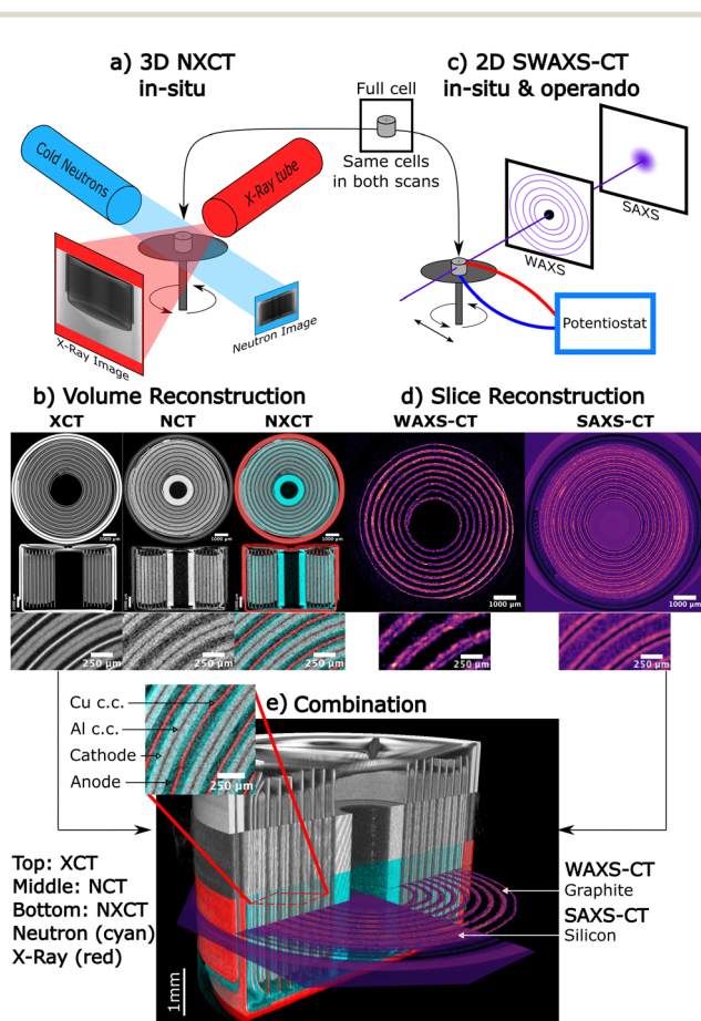
Fig. 1 Methodology for the multimodal 3D correlative visualization. (a) Schematic of the neutron and X-ray computed tomography (NXCT) set-up for in situ measurement. NCT and XCT scans were done sequentially. (b) Slices through the reconstructed tomography volumes of the cell. The left part shows XCT data, the middle part shows the NCT data in the identical position and the right part shows the combined NXCT images in false color, with the red component corresponding to X-ray attenuation and the cyan component corresponding to neutron attenuation. Top row: Horizontal slices through the 3D volume. Middle row: vertical slices providing a complementary side view of the internal structure and casing. Bottom rows: Detailed view of the rolled electrode structure. (c) Schematic of the small angle and wide angle scattering computed tomography (SWAXS-CT) measurement setup. (d) Reconstructed 2D SWAXS-CT slices. Left part: Integrated graphite intensity between q = 1.82\text{--}1.92 \text{ \AA}^{-1} . Right part: Integrated SAXS intensity between q = 0.025\text{--}0.1 \text{ \AA}^{-1} . Bottom: Detailed view showing the anode layers as purple-enhanced regions. (e) Multimodal correlative data and 3D rendering of the cell. Top part: X-ray CT data. Middle part: Neutron CT data. Bottom part: Combined NXCT data in false color. A 2D SWAXS CT slice is also shown in the measured position. Right: Integrated graphite intensity. Left: Integrated SAXS intensity. The insert highlights the various components and internal cell damage as observed with NXCT.
