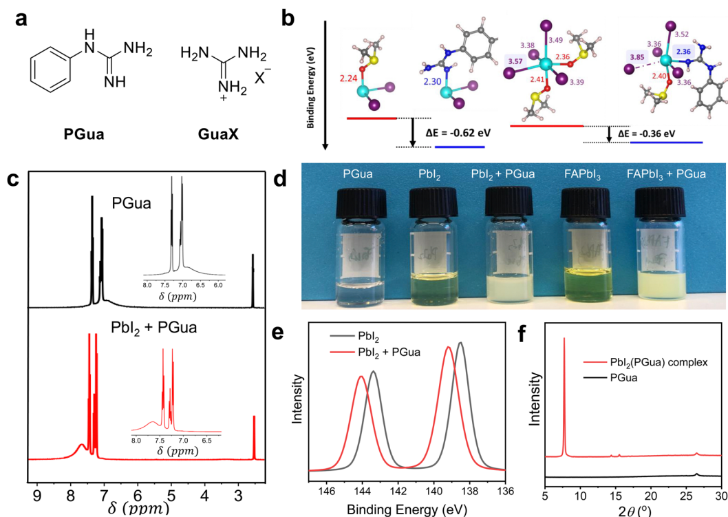
Fig. 1 The interaction of \text{PbI}_2 and PGua (a) chemical structure of PGua and GuaX; (b) binding energy of DMSO and PGua with \text{PbI}_2 precursor complexes. Replacement of DMSO with PGua in a high-valent iodoplumbate [\text{PbI}_4]^{2-} results in the release of iodide ions. The following color code is used for the atomic representations: purple, I; cyan, Pb; blue, N; red, O; yellow, S; gray, C; pinkish white, H. Distances between ligands and iodide and the Pb center are given in units of Å, highlighted in the color of the respective species. (c) ^1\text{H} NMR spectra of PGua solution and the mixed solution of PGua and \text{PbI}_2 , which were dissolved in \text{DMSO}-d_6 ; (d) photos of different DMSO solutions, the concentration in all cases is 0.1 M; (e) XPS core level signals of Pb 4f of \text{PbI}_2 film and of \text{PbI}_2(\text{PGua}) complex film; (f) XRD patterns of PGua and \text{PbI}_2(\text{PGua}) complex films. The molar ratio of PGua and \text{PbI}_2 is 1:1 in the above experiments (e) and (f).
