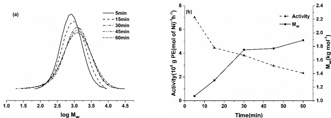
Fig. 5 (a) GPC curves of the polyethylene produced using Ni5/EASC over different reaction times; (b) effects of reaction time on the catalytic activity and molecular weight of polyethylene (entries 6 and 9–12, Table 3).
