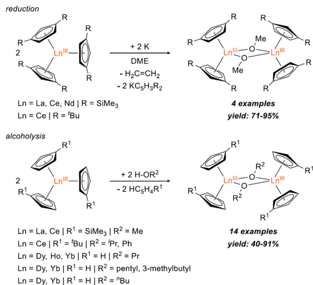
Fig. 1 Reported syntheses of [\text{Cp}^{\text{R}}_2\text{Ln}(\mu\text{-OR})_2] bimetallic complexes via reduction 28,29 (top) and alcoholysis 31–35 (bottom).
