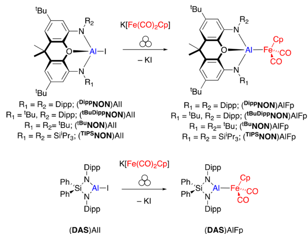
Fig. 2 Solid-state structures of ( Dipp NON)AlFp (top-left), ( t BuDipp NON)AlFp (top-right), ( t Bu NON)AlFp (middle-left), ( TIPS NON)AlFp (middle-right) and (DAS)AlFp (bottom) as determined by single-crystal X-ray crystallography. Displacement ellipsoids set at the 50% probability level. Hydrogen atoms have been omitted and selected organic groups have been shown in wireframe for clarity.
