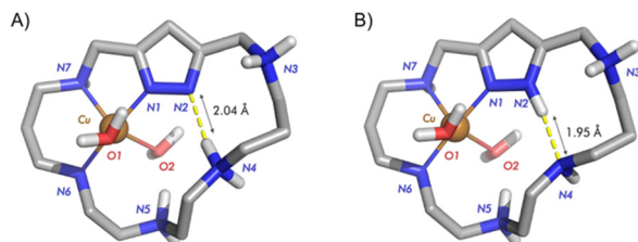
Fig. 5 Representation of the most stable structure for the diprotonated \text{Cu}^{2+} - L1 complex. (A) [\text{Cu}(\text{H}_3(\text{H}_{-1}\text{L1}))]^{4+} and (B) [\text{Cu}(\text{H}_2\text{L1})]^{4+} . Structure B is ca. 1.0 \text{ kJ mol}^{-1} more stable than A.
