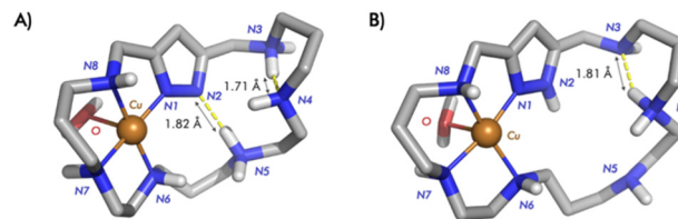
Fig. 6 Representation of the most stable structure for the monoprotonated \text{Cu}^{2+} - L2 complex. (A) [\text{Cu}(\text{H}_2(\text{H}_{-1}\text{L2}))]^{4+} and (B) [\text{Cu}(\text{HL2})]^{4+} . Structure B is ca. 25.3 \text{ kJ mol}^{-1} more stable than A.
