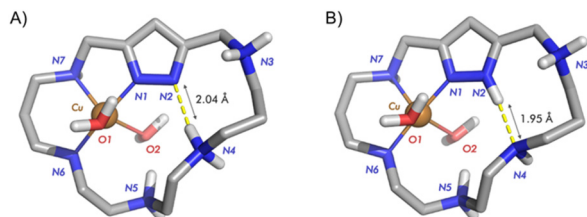
Fig. 4 Representation of the most stable structure for the monoprotonated \text{Cu}^{2+} - L1 complex. (A) [\text{Cu}(\text{H}_2(\text{H}_{-1}\text{L1}))]^{3+} and (B) [\text{Cu}(\text{HL1})]^{3+} . Structure B is ca. 8.8 \text{ kJ mol}^{-1} more stable than A.
