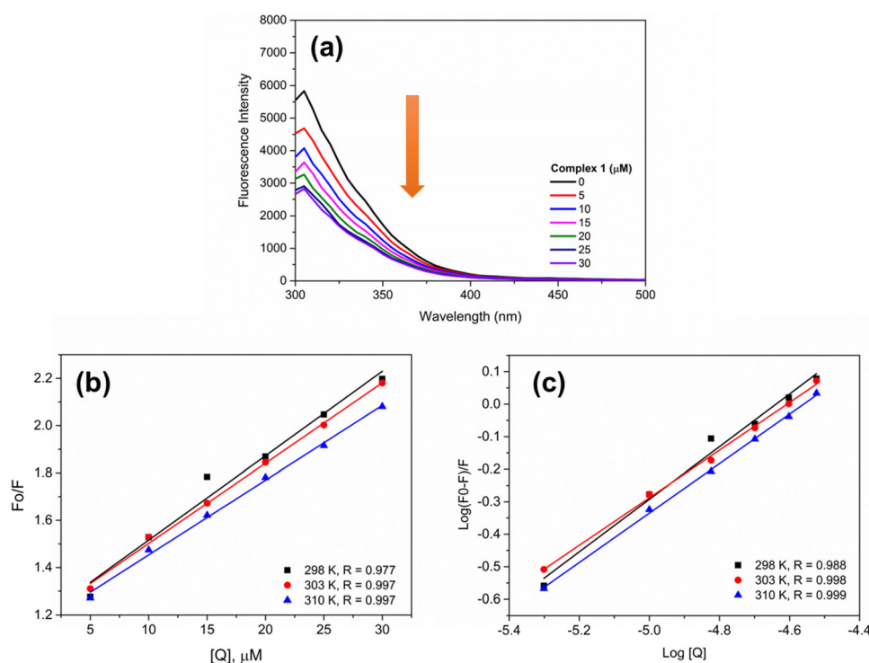
Fig. 6 (a) Fluorescence spectra of HSA (5 \mu\text{M} , \lambda_{\text{ex}} = 270 \text{ nm} ) in the absence and presence of 1 at different concentrations. (b) Stern–Volmer plot and (c) plot of \log[(F_0 - F)/F] vs. \log[Q] , at 298, 303 and 310 K.
