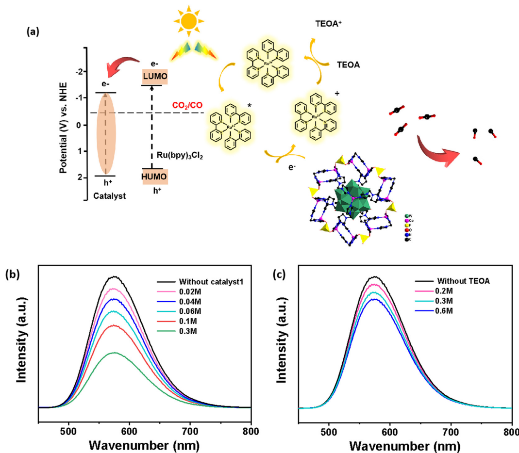
Fig. 4 (a) The speculative mechanism for the photocatalytic CO 2 reduction by Co-PO 4 -PW 12 . (b and c) The photoluminescence spectra of MeCN solution in the presence of [\text{Ru}(\text{bpy})_3]\text{Cl}_2 obtained with different doses of Co-PO 4 -PW 12 (0.02 M–0.3 M) and TEOA (0.2 M–0.6 M).
