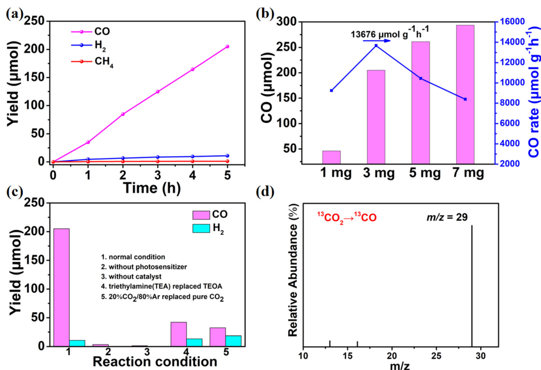
Fig. 3 (a) Production of CO over time is depicted on a trend line, (b) the effect of quantity on the production of CO, (c) the study of the \text{CO}_2 RR under varied situations, and (d) the mass spectra in the ^{13}\text{CO}_2 isotopic detection experiment over Co-PO 4 -PW 12 as a photocatalyst.
