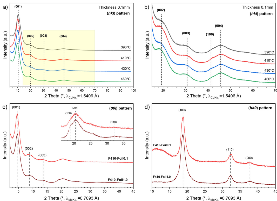
Fig. 2 (a) XRD patterns of fluorinated graphite foils ( \text{Cu} \text{K}\alpha radiation with \lambda_{\text{CuK}\alpha_1} = 1.5406 \text{ \AA} ) and (b) with magnification in the 15\text{--}70^\circ 2\theta range (shown as a yellow area on (a)). (c) and (d) are respectively the (00 l ) and ( hk0 ) patterns of foils of 0.1 (F410-Foil0.1, red) and 1.0 mm (F410-Foil1.0, dark red) thickness fluorinated at 390^\circ\text{C} and then annealed under \text{F}_2 gas at 410^\circ\text{C} . The latter were acquired with a Mo \text{K}\alpha source ( \lambda_{\text{MoK}\alpha_1} = 0.7093 \text{ \AA} ).
