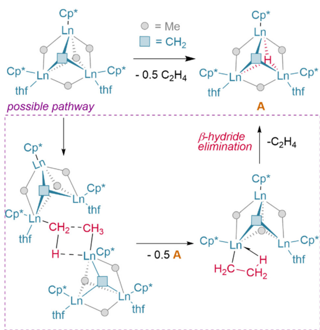
Fig. 7 Spontaneous \text{C}=\text{C} bond formation from a lanthanide alkyl/alkylidene complex may proceed via \beta -hydride elimination to yield the \mu^3 -hydride product (A).
