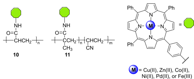
Fig. 5 M10 ( M = \text{Zn(II)}, \text{Cu(II)}, \text{Ni(II)}, \text{Co(II)}, \text{Fe(III)}, \text{and Pd(II)} ) and Fe11 supported in a polyacrylonitrile or polyacrylonitrile copolymer nanofibre mat.
