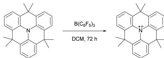
Scheme 2 The first reported example of an SET between \text{B}(\text{C}_6\text{F}_5)_3 and an organic electron donor, in this case a triarylamine, as reported by Wang et al.
