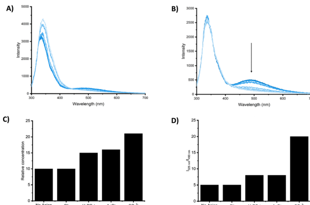
Fig. 30 Emission spectra of 87 (20 \mu\text{M} ) in DMSO (1% \text{H}_2\text{O} ) upon addition of \text{TBA}_2\text{SO}_4 (0 to 60 equiv.) ( \lambda_{\text{exc}} = 280 nm) at 298 K (A). Emission spectra of 88 (20 \mu\text{M} ) in DMSO/1% \text{H}_2\text{O} upon addition of \text{TBA}_2\text{SO}_4 (0 to 80 equiv.) ( \lambda_{\text{exc}} = 280 nm) at 298 K (B). The ratios of I_{325}/I_{490} for 87 (C) and 88 (D) in DMSO/1% \text{H}_2\text{O} at 298 K in the presence of anion (10 equiv.). Adapted with permission from ref. 82. Copyright RSC 2023.
