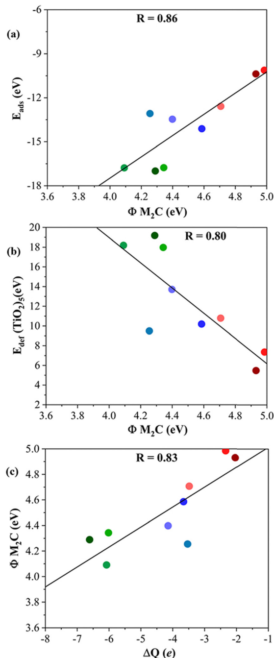
Fig. 7 (a) E_{ads} vs. the work function, \Phi , of bare (0001) MXene surfaces; (b) E_{def}(TiO_2)_5 vs. \Phi M_2C ; and (c) \Phi M_2C vs. \Delta Q of (TiO_2)_5 . The solid black lines correspond to the linear fitting associated with the regression coefficient, R . Color coding as in Fig. 3. Linear fitting analysis is reported in Table S12 of the ESI†
