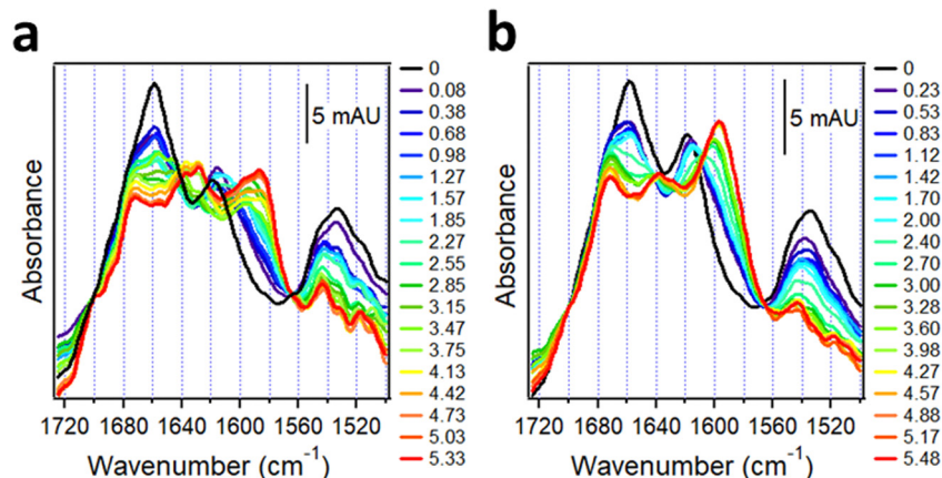
Fig. 7 Structural changes in ^{13}\text{C} - \text{A}\beta_{1-42} and \text{A}\beta_{\text{pE3-42}} upon hydration with \text{D}_2\text{O} -saturated nitrogen gas when physically separated (a) and combined at 1:1 molar ratio (b). Both panels are appended with columns indicating time of exposure to \text{D}_2\text{O} vapor (in hours). Reproduced from ref. 37, with permission.
